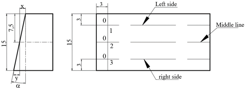
Figure 4. Measurement coordinates of the surface roughness and waviness of the cut workpiece at different longitudinal feed rates
